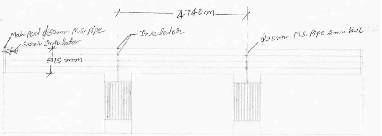
Sketch for Solar fencing
